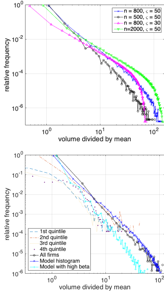
FIGURE 2.— Histograms of volume normalized by its time-series average. Top : Histograms of equilibrium volume M_n^\dagger for various parameter values, where n is the number of traders and \zeta is the standard deviation of private information. Bottom : Daily volume histograms for individual stocks and a pooled sample, plus simulated histograms. Data for individual firms cover 1988–2018. Data for the pooled sample is for 2016. Individual firms are selected at the quintiles of market capitalization size in the TSE. The circle-line shows the histogram of pooled data for all listed firms. The cross-line shows a simulated histogram with n = 800 and \zeta = 50 . The plus-line shows the case with a higher \beta .
