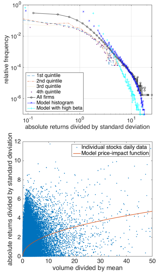
FIGURE 3.— Top : Histograms of the absolute values of daily returns. The horizontal axis shows the daily return, which is the difference in logarithm of opening and closing prices for each business day. The samples are the same as in Figure 2. Bottom : A scatter plot of daily volume and absolute returns for all listed firms in 2016. The red line shows the price-impact function fitted by non-linear least squares.
